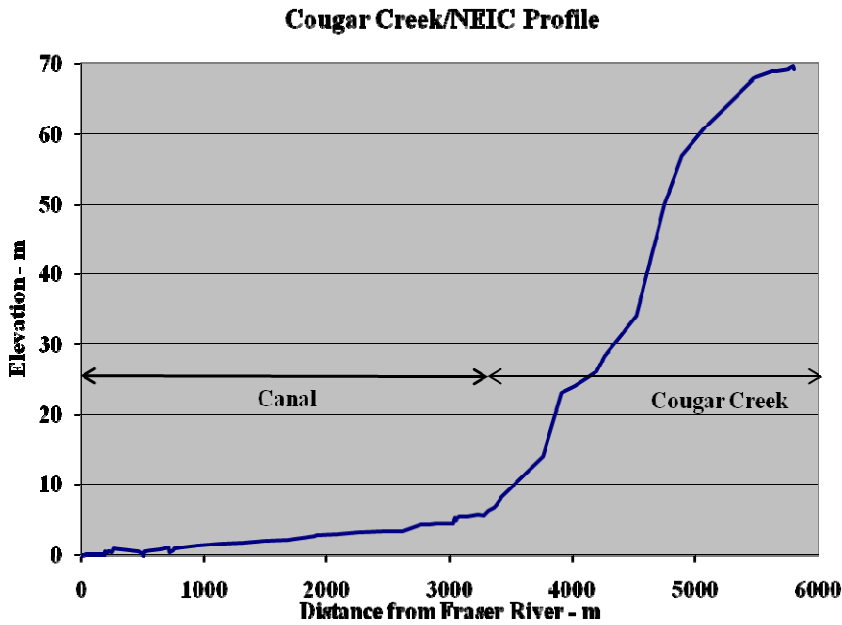
Figure 3-11: Bed Profile of the Cougar Creek/NEIC System
