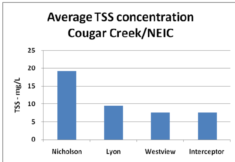
Figure 2-10: Average TSS Concentrations at Four Sample Sites
