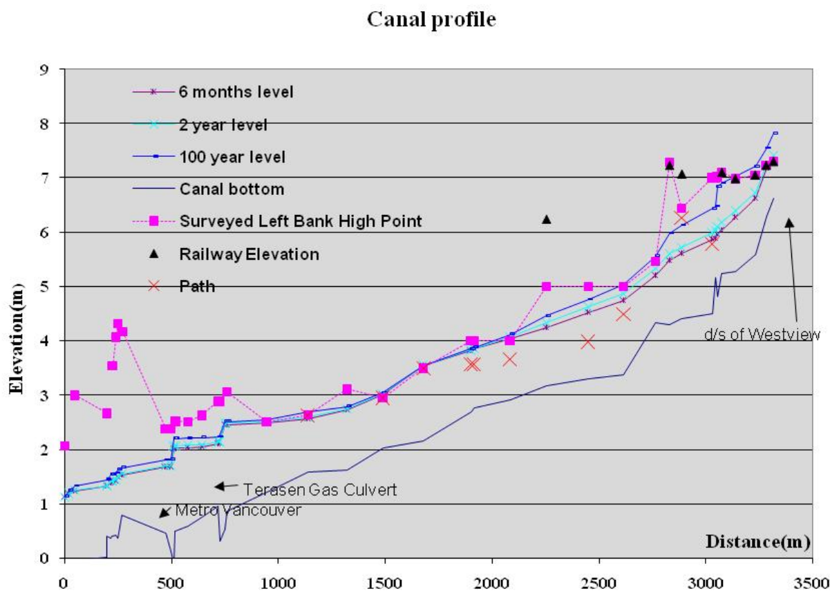
Figure 3-13: Canal Profile
