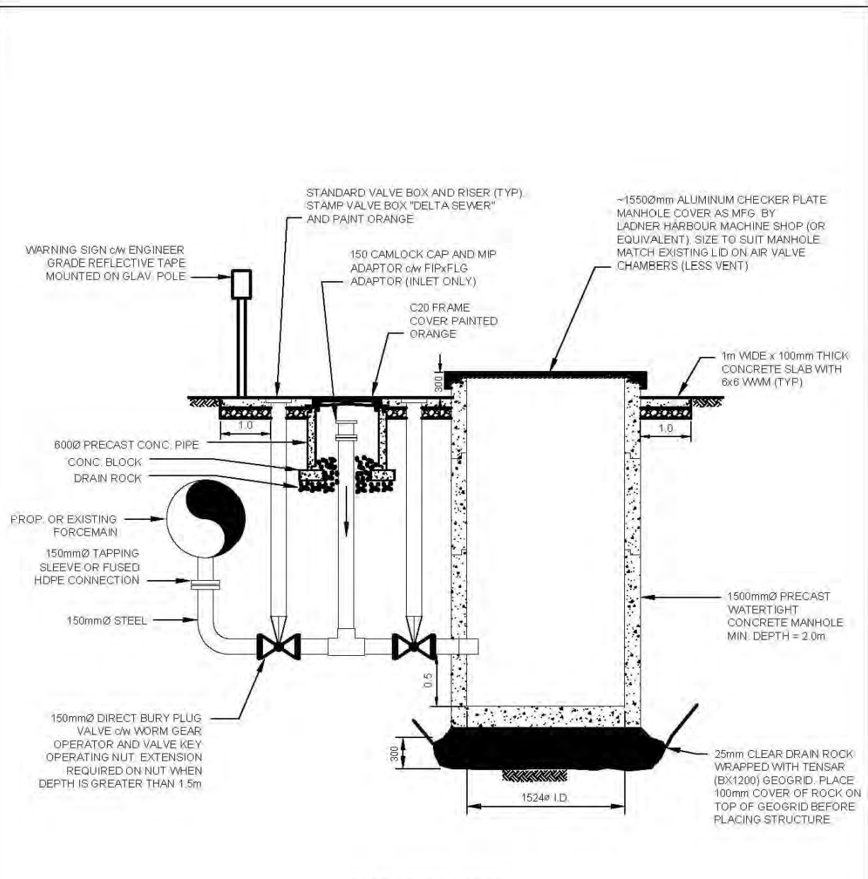
ELEVATION VIEW NTS
