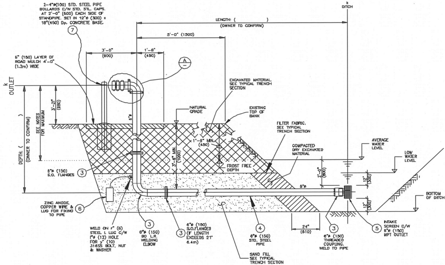
SECTION THRU' STANDPIPE
